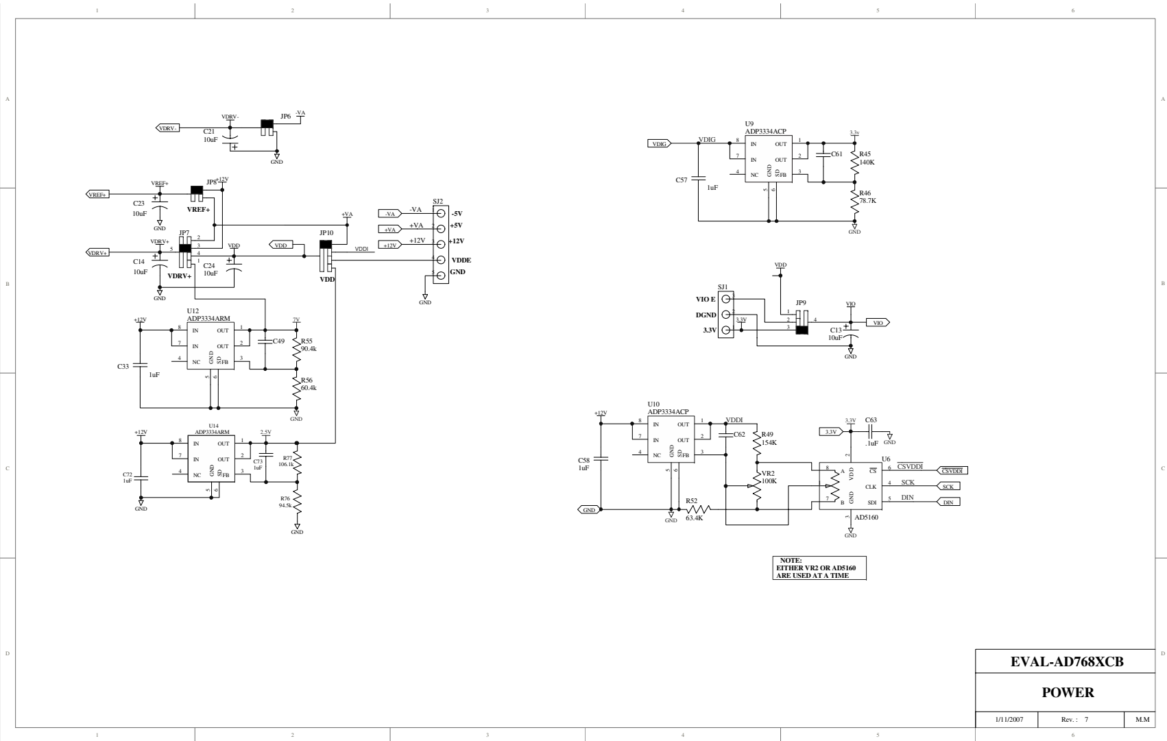
Figure 4. Schematic (Power Section)
