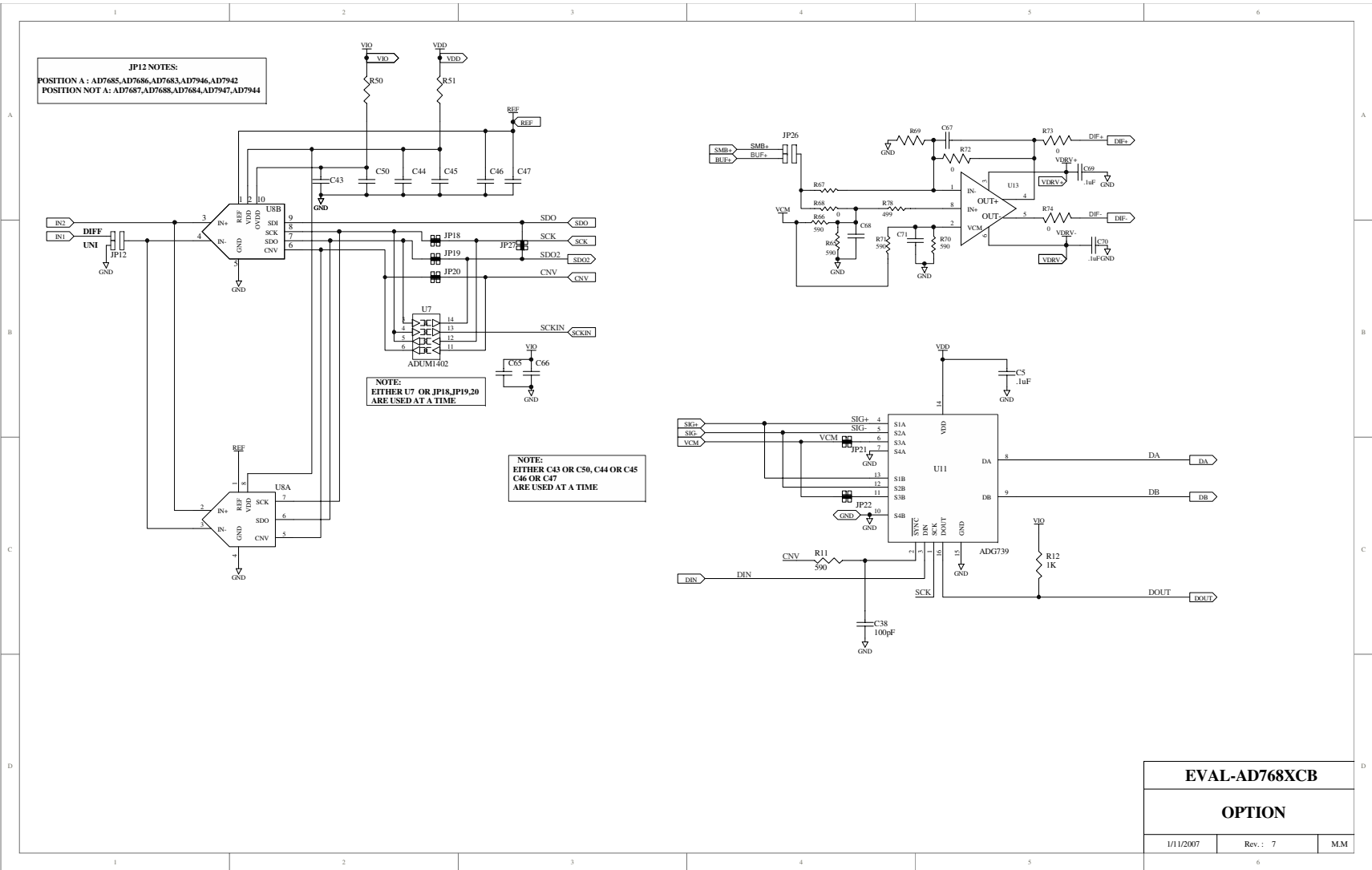
Figure 5. Schematic (Option Section)
