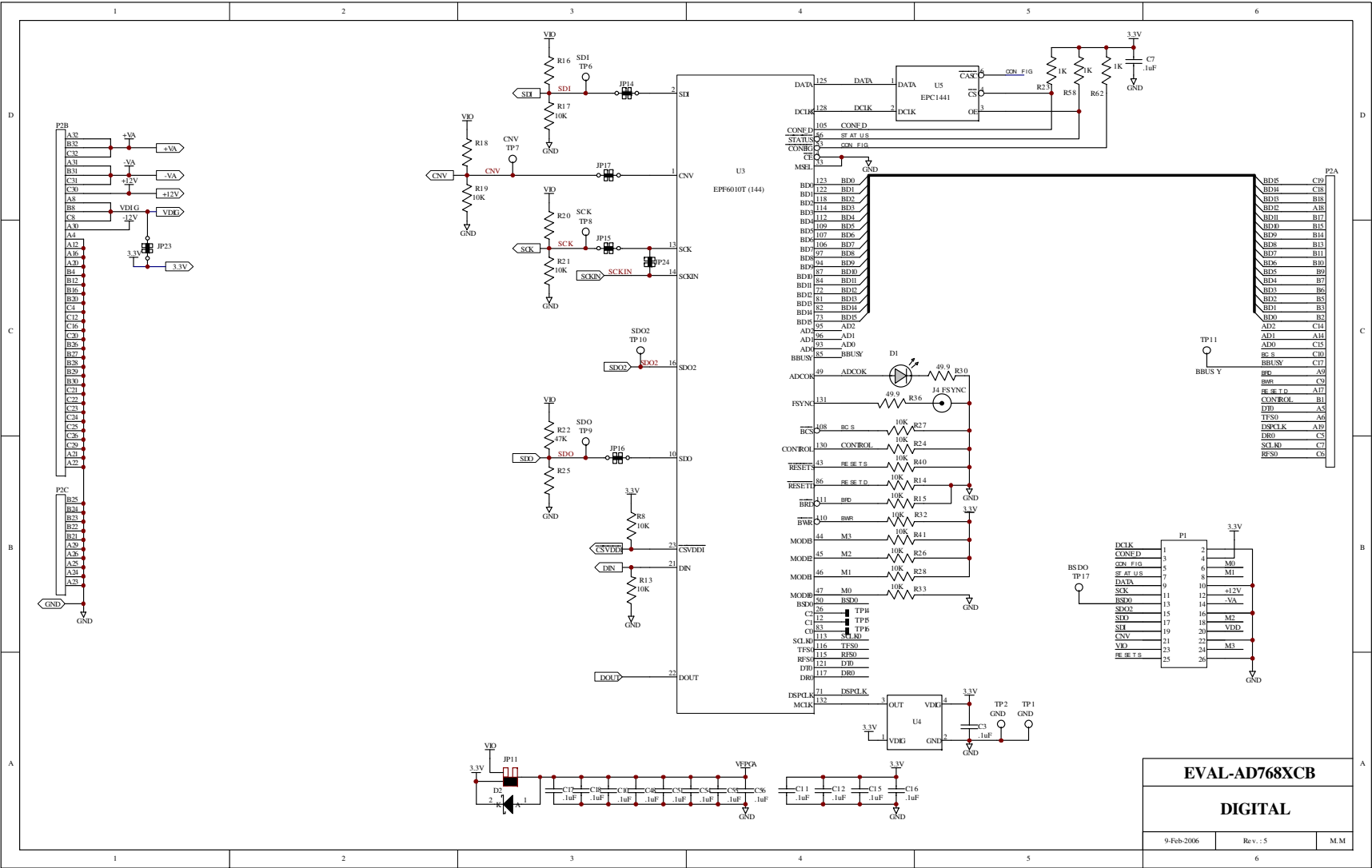
Figure 3. Schematic (Digital Section)
