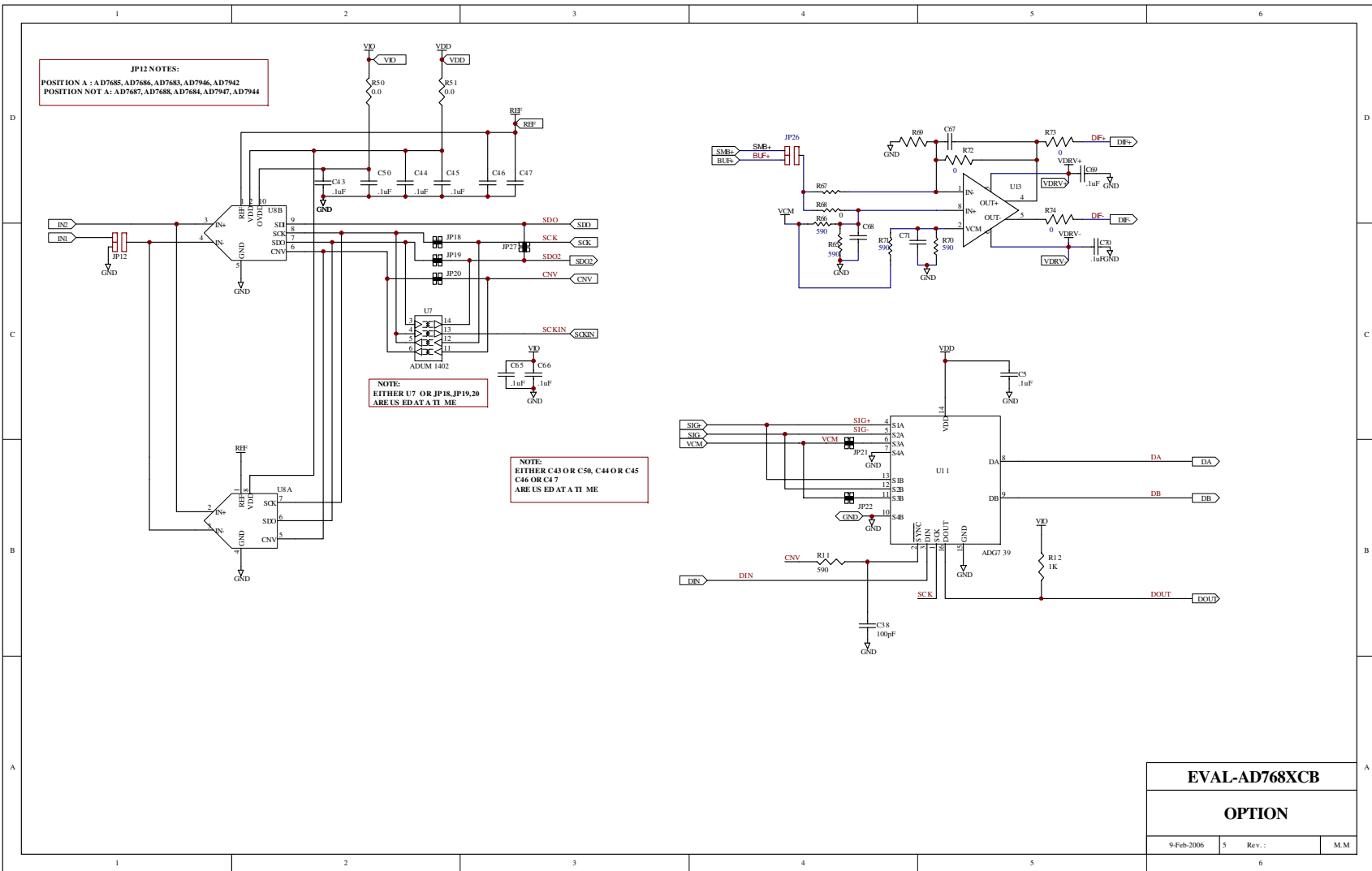
Figure 4. Schematic (Option Section)
