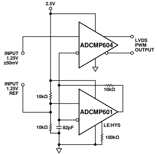
Figure 25. Oscillator and Pulse-Width Modulator
