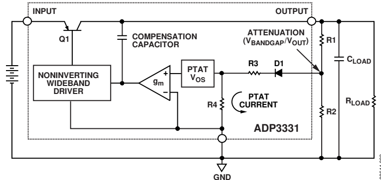
Figure 3. ADP3331 Functional Diagram
