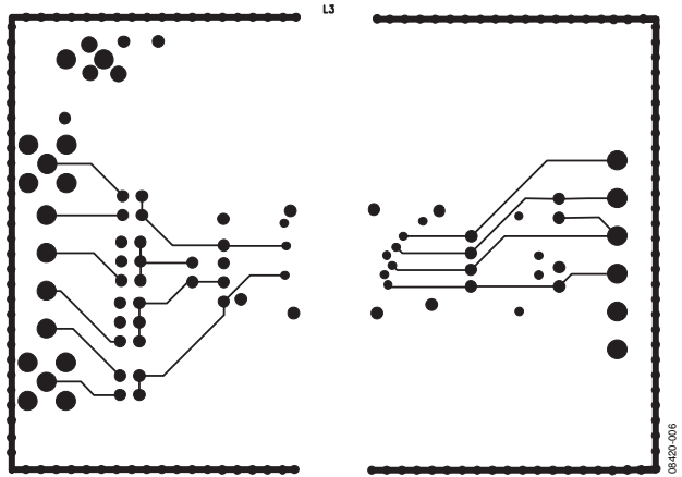
Figure 7. Internal Layer 3
