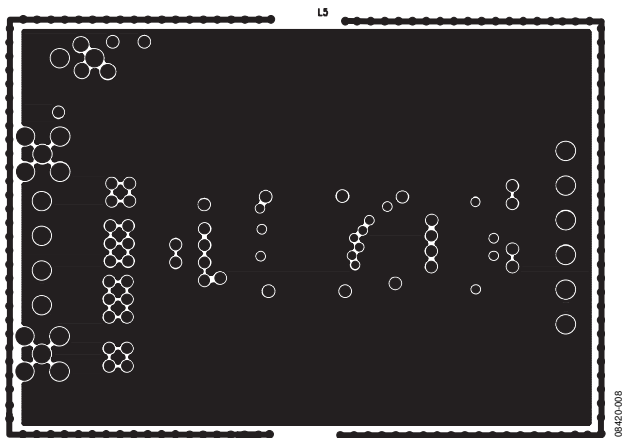
Figure 9. Internal Layer 5
