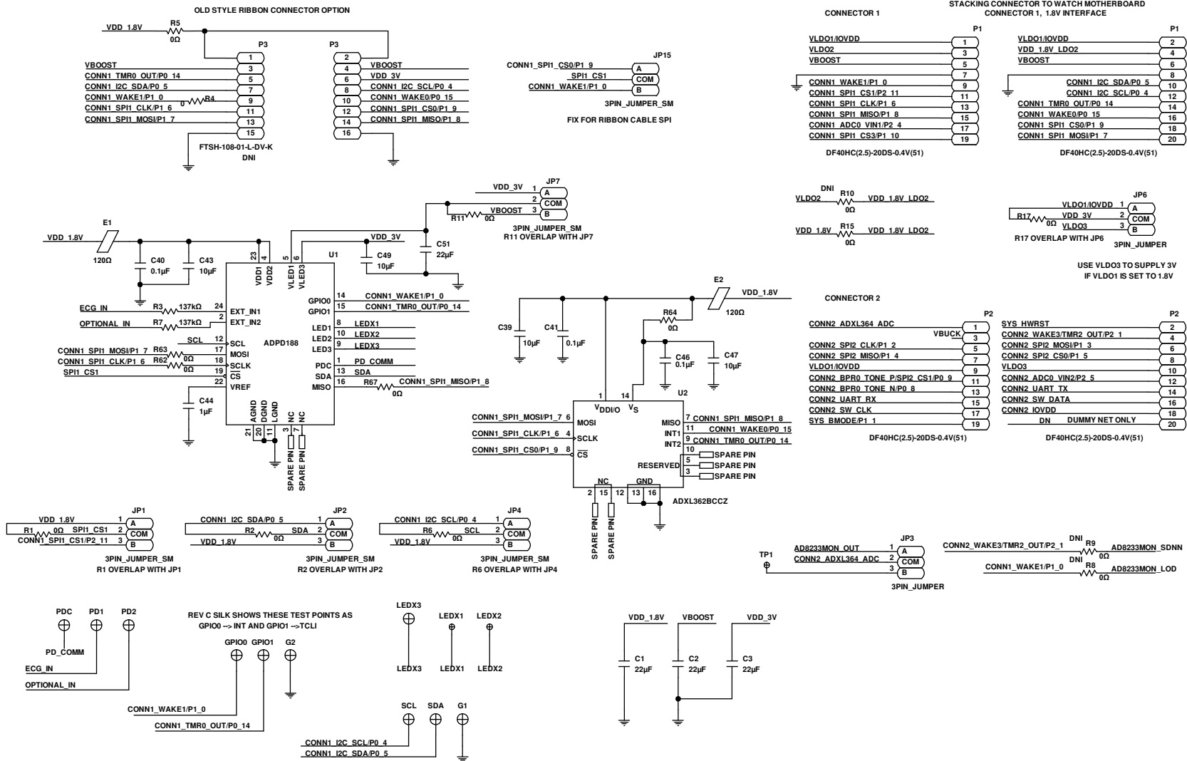
Figure 13. EVAL-ADPD188GGZ Schematic
