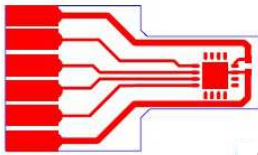
Figure 22. ADT7320FBZ Component Side (Layer 1)
