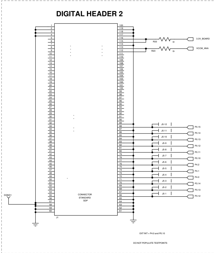
Figure 9. Digital Schematics 2
