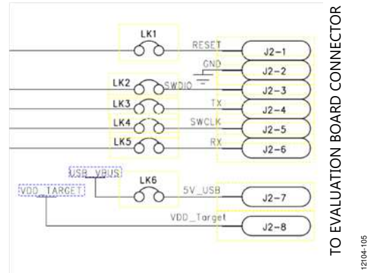
Figure 5. J2 Connector
