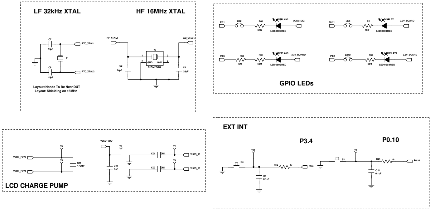
Figure 8. Digital Schematics 1
