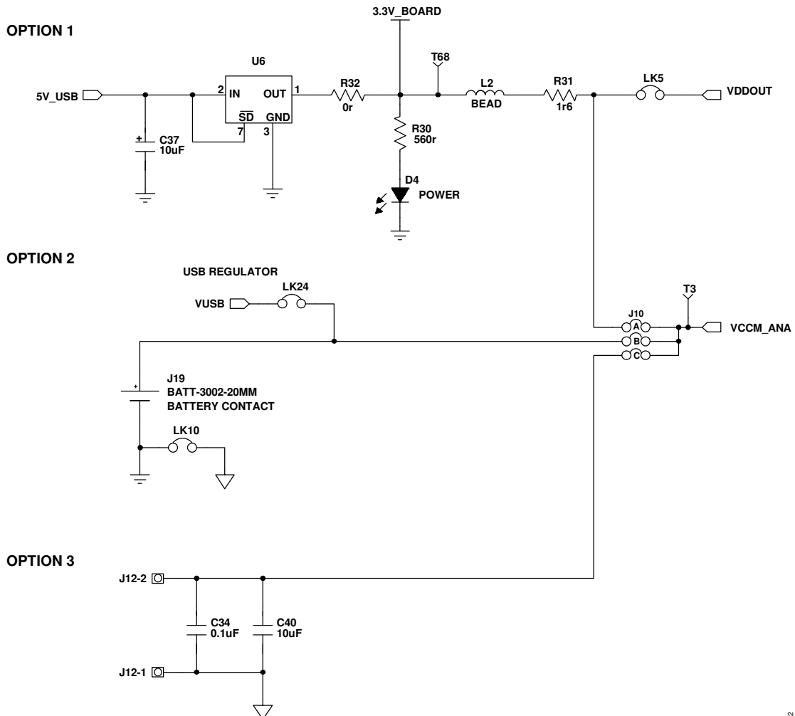
Figure 3. Power Supply Schematic for VCCM_ANA Pin Rev. 0 | Page 5 of 28
