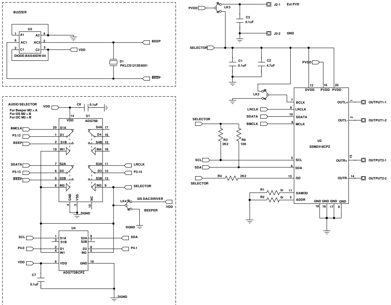
Figure 20. Audio Schematic
