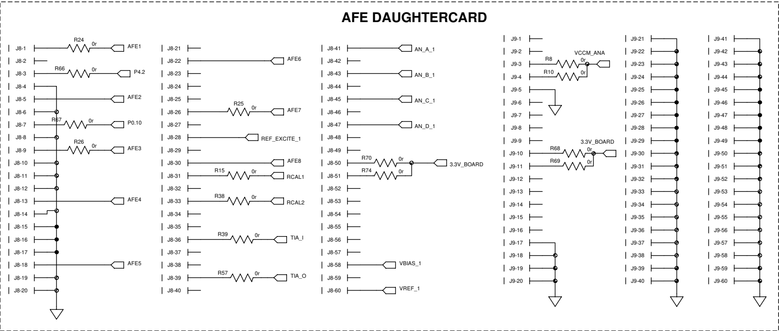
Figure 10. Analog Schematics 1
