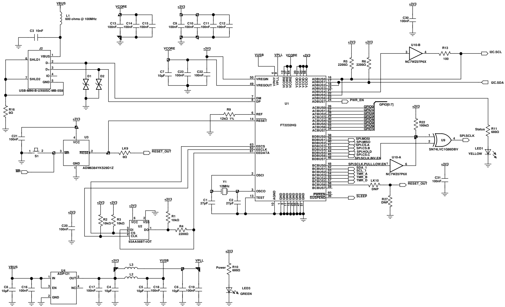
Figure 8. SDP-S—USB-to-Serial Engine, USB, Interface
