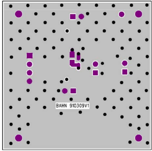
Figure 11. Bottom Layer
