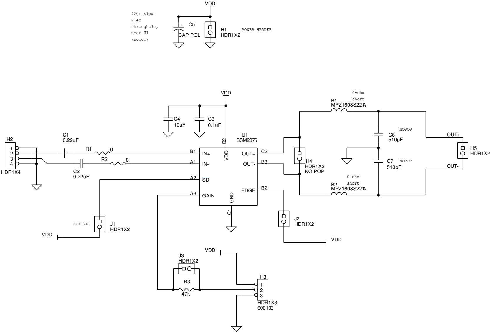
Figure 3. Schematic of the SSM2375 Evaluation Board Rev. 0 | Page 6 of 8
