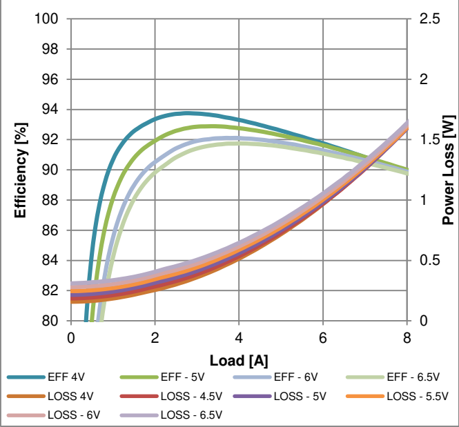
Figure 8: Efficiency – V_{OUT} = 1.8V , various V_{OUT} , T = -40^{\circ}C
