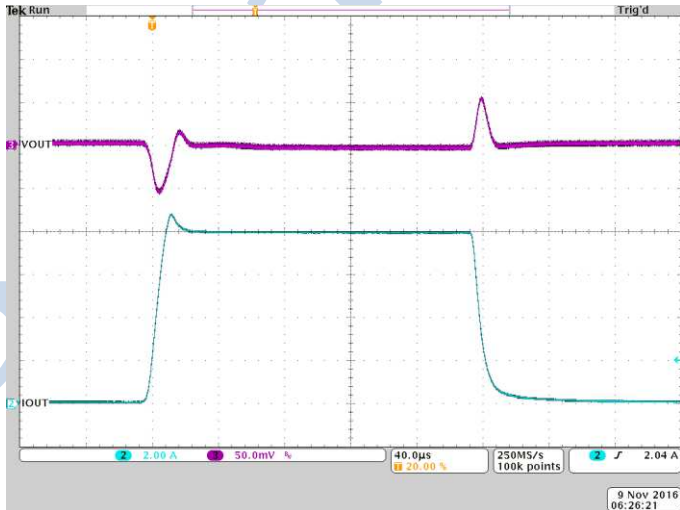
Figure 20: 0/8A load transient
