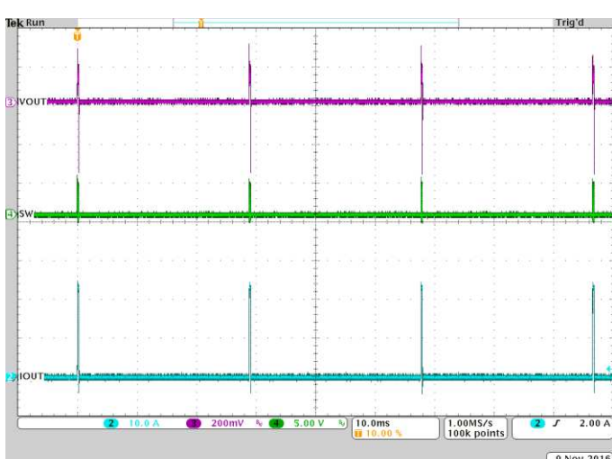
Figure 22: Hiccup mode during short-circuit protection
