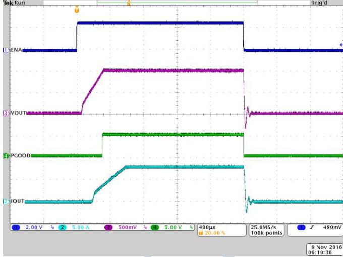
Figure 18: Startup V_{IN} = 5V , V_{OUT} = 1V , I_L = 8A
