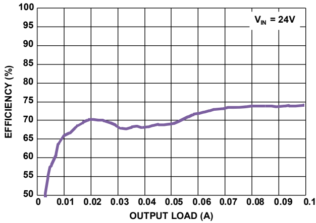
FIGURE 23. EFFICIENCY vs LOAD, PFM, V_{OUT} = 1.8\text{V}
