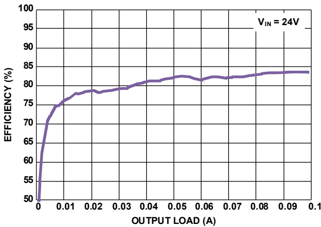
FIGURE 25. EFFICIENCY vs LOAD, PFM, V_{OUT} = 5\text{V}
