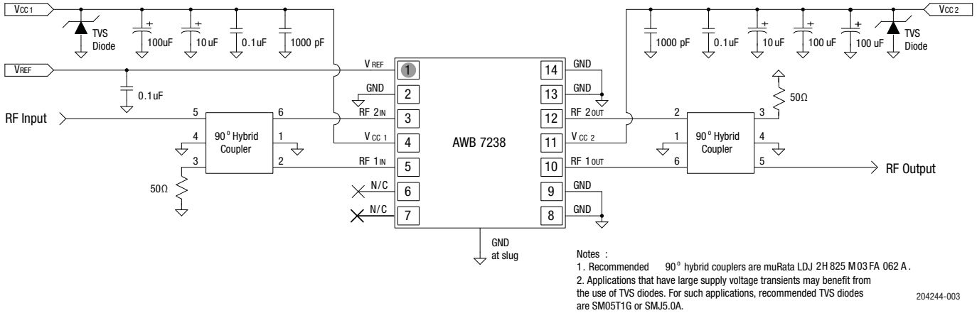
Figure 3. AWB7238 Application Circuit Schematic
