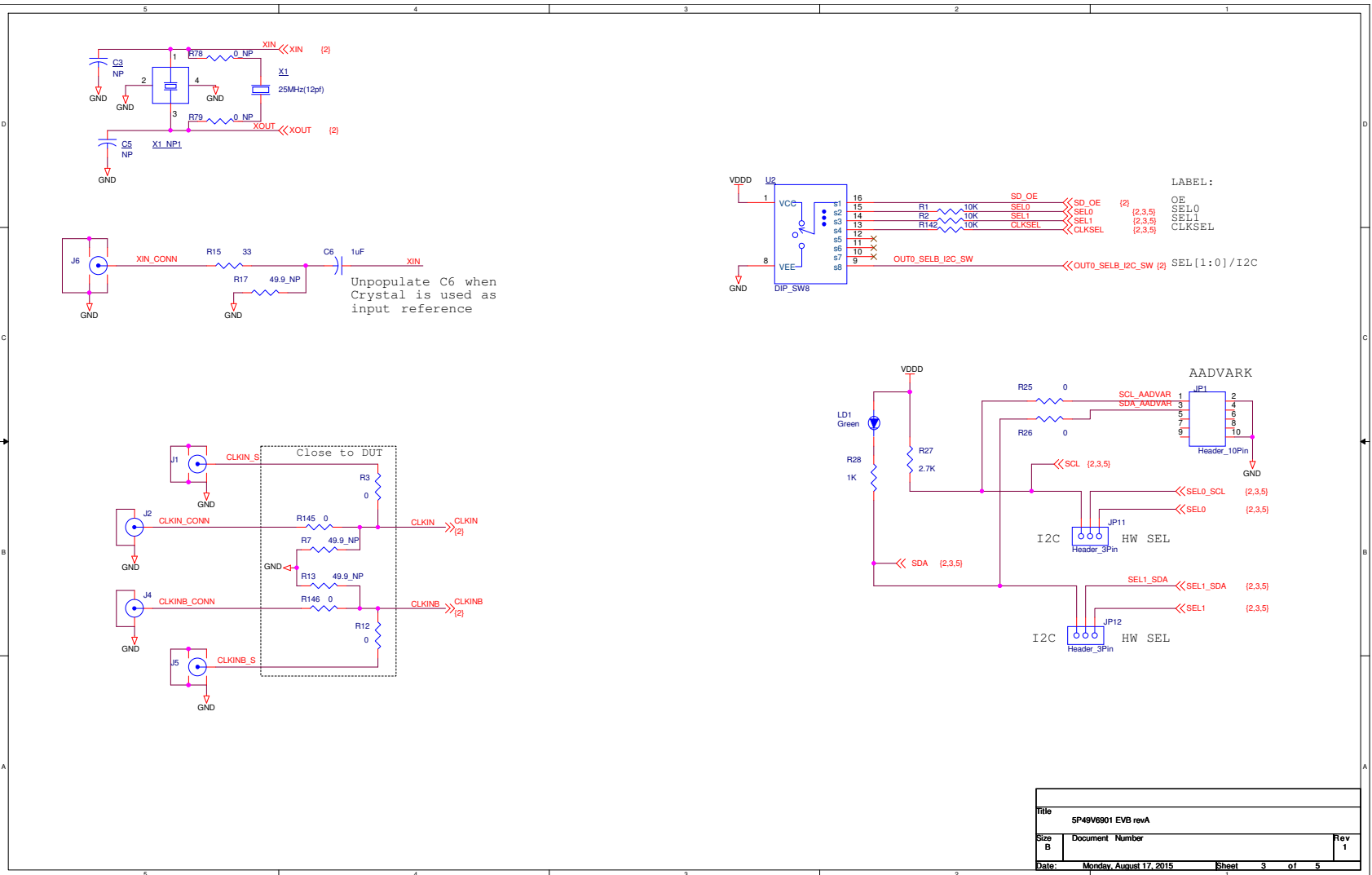
Figure 6. 5P49V6901 VersaClock 6 Evaluation Board Schematics – Page 2
