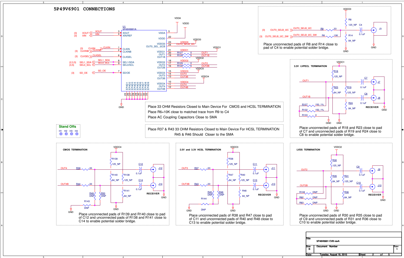
Figure 5. 5P49V6901 VersaClock 6 Evaluation Board Schematics – Page 1
