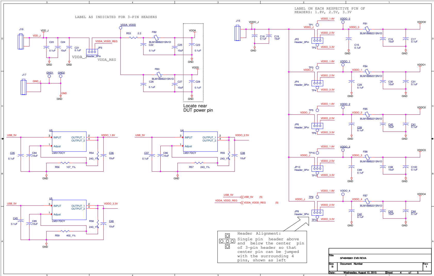
Figure 7. 5P49V6901 VersaClock 6 Evaluation Board Schematics – Page 3
