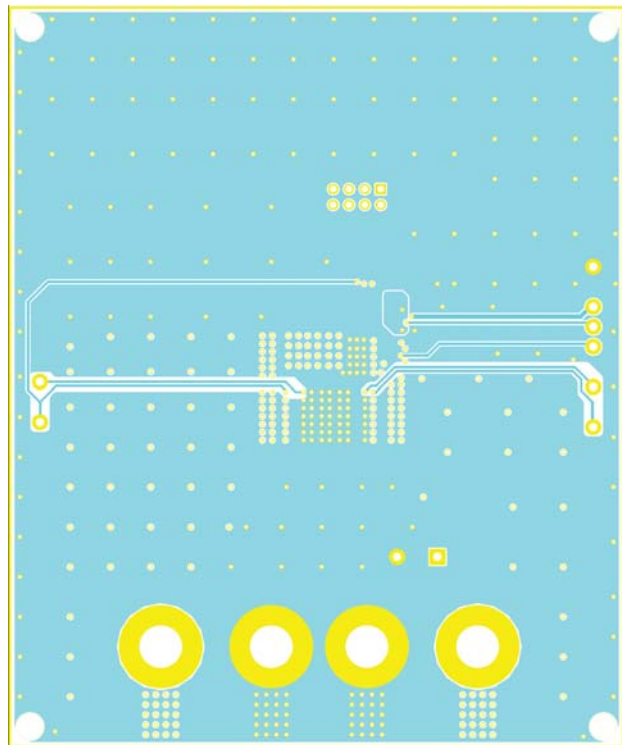
Figure 3: Inner Layer 2
