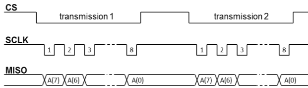
Figure 10: Timing Diagram for Simple SPI Readout
