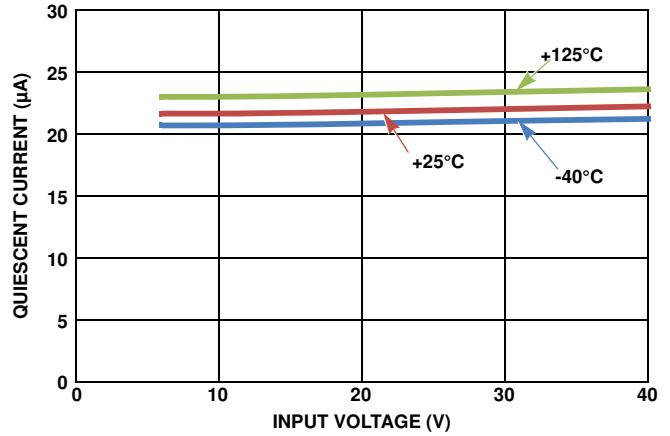
FIGURE 4. QUIESCIENT CURRENT vs INPUT VOLTAGE (NO LOAD)
