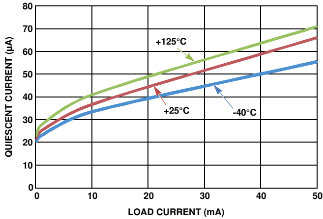
FIGURE 3. QUIESCIENT CURRENT vs LOAD CURRENT
