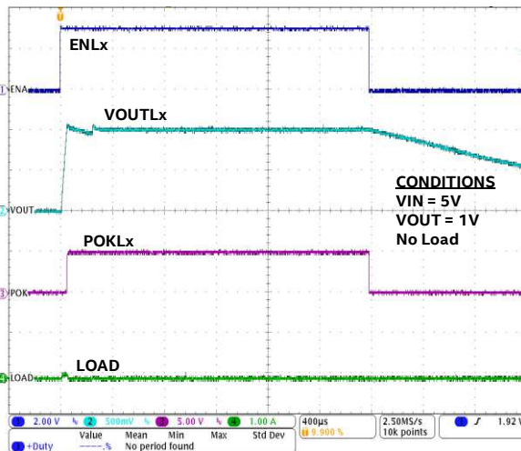
LDO Startup and Shutdown
