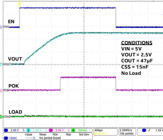
Buck Startup and Shutdown
