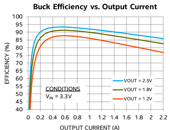
Figure 2: Efficiency at VIN = 3.3V
