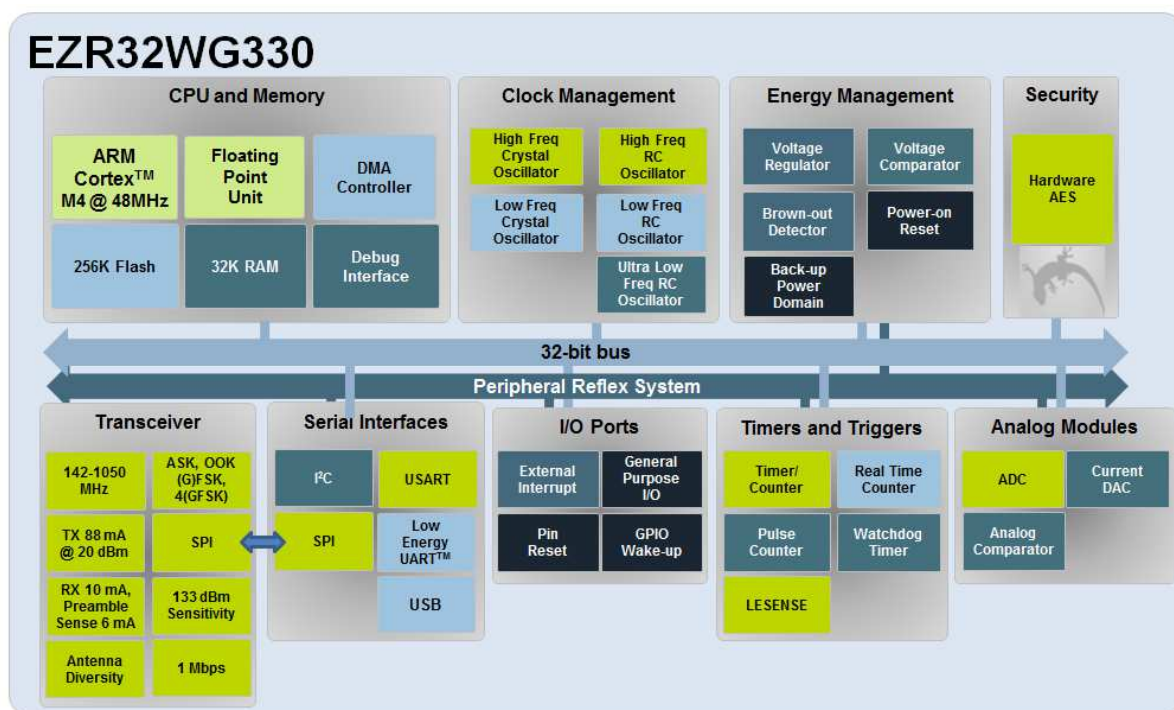
Figure 3.1. Block Diagram
