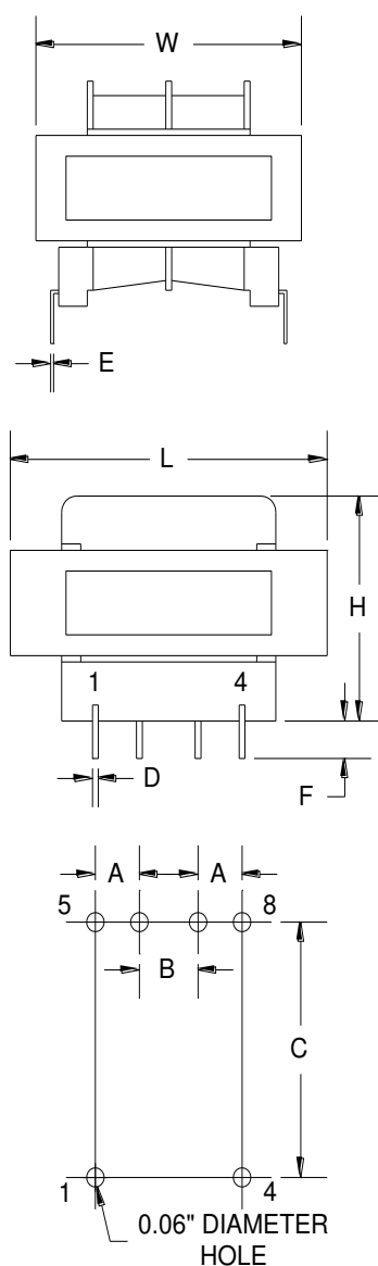
Board Layout
