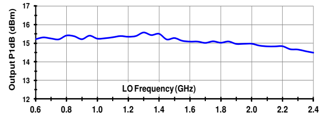
1dB Compression
