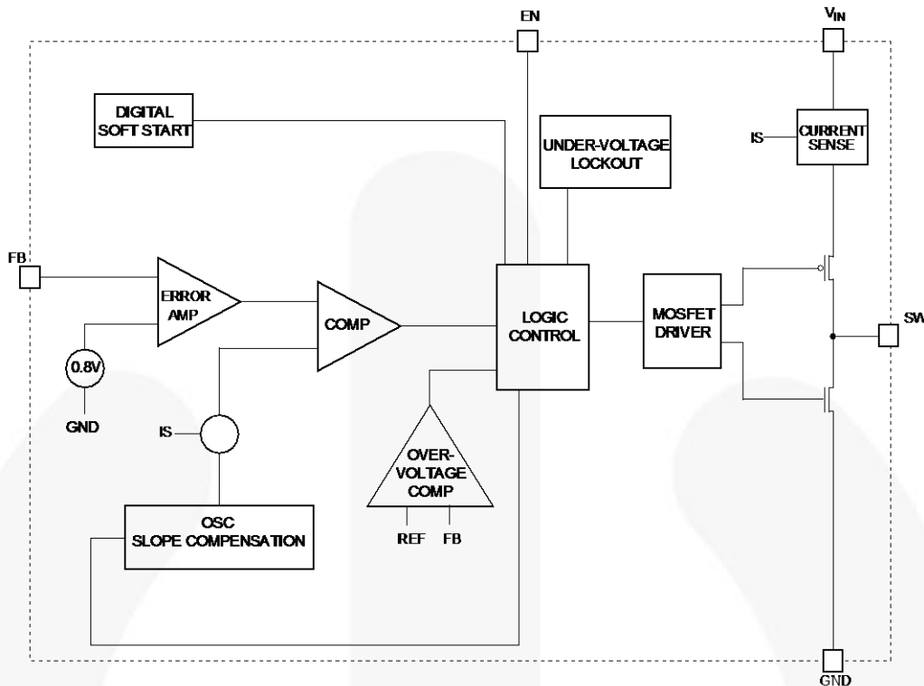
Figure 13. Block Diagram
