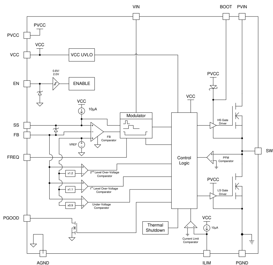
Figure 2. Block Diagram
