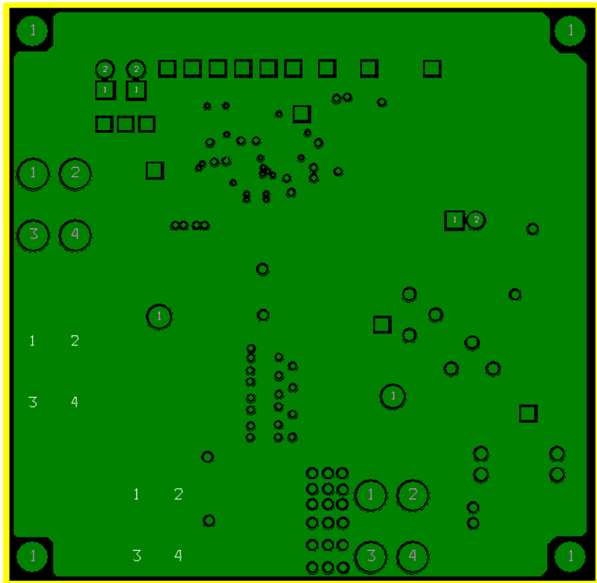
Figure 27. Evaluation Board Inner Layer 2 Copper
