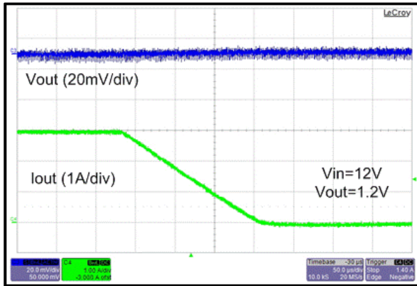
Figure 24. FAN23SV06PA Operation as Load Changes from 3 A to 0 A
