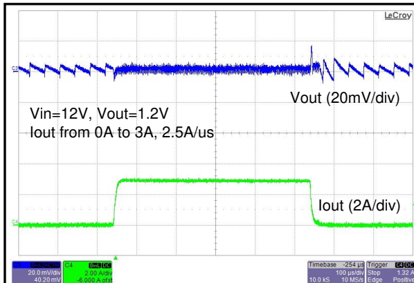
Figure 26. FAN23SV06A Load Transient from 0% to 50% Load Current
