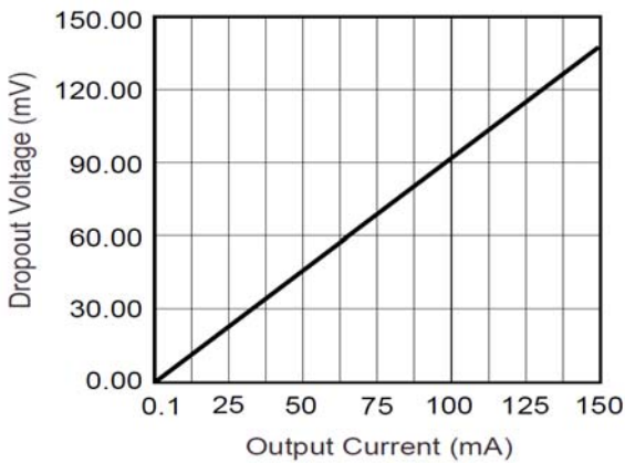
Figure 19. Dropout Voltage
