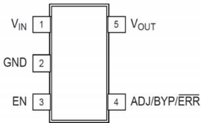
Figure 2. Pin Configuration
