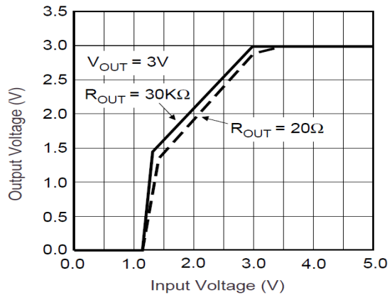
Figure 20. Dropout Characteristics
