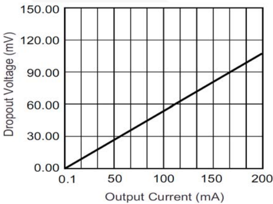
Figure 19. Dropout Voltage
