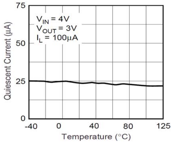
Figure 15. Ground Pin Current
