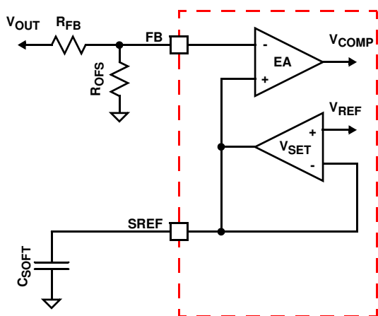
FIGURE 9. ISL95870 VOLTAGE PROGRAMMING CIRCUIT
