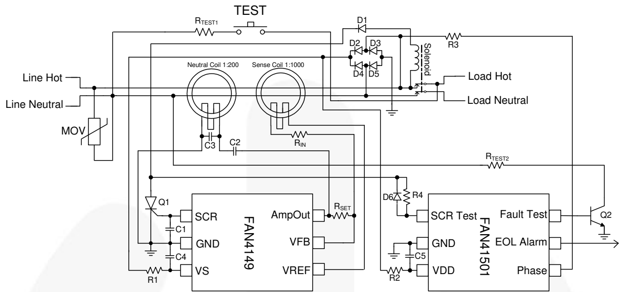
Figure 1. Typical Application (1,2)
