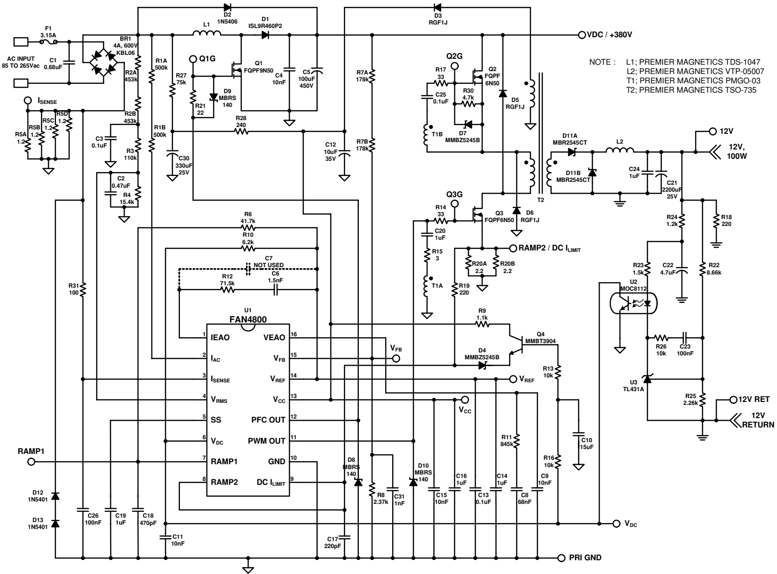
Figure 12. Current-Mode Application
