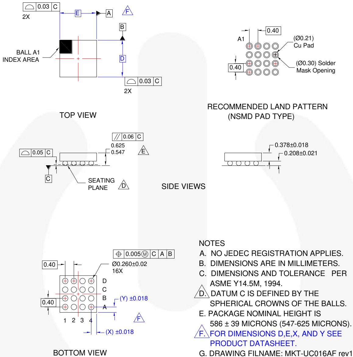
Figure 25. 16-Ball, 4x4 Array, 0.4 mm Pitch, 250 µm Ball, Wafer-Level Chip-Scale Package (WLCSP)
