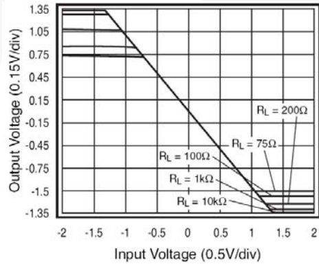
Figure 17. Output Swing vs. Load
