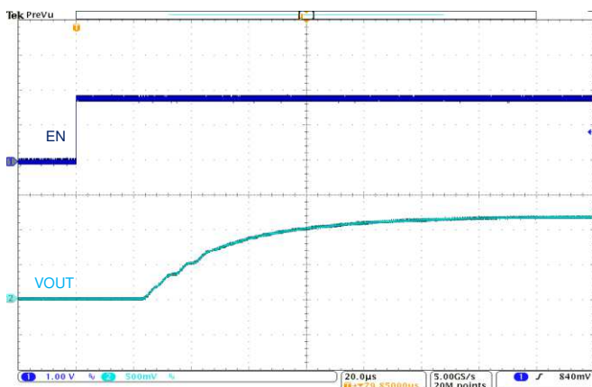
Figure 17. Startup, 5 \Omega Load, V_{OUT} = 1.15625\text{ V} , V_{IN} = 3.6\text{ V}
