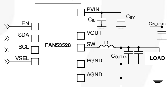
Figure 1. Typical Application
