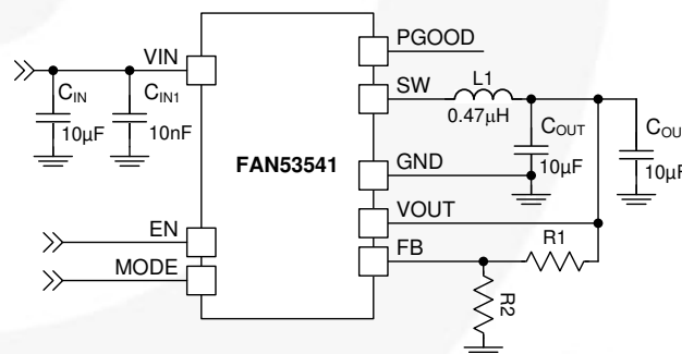
Figure 1. Typical Application
