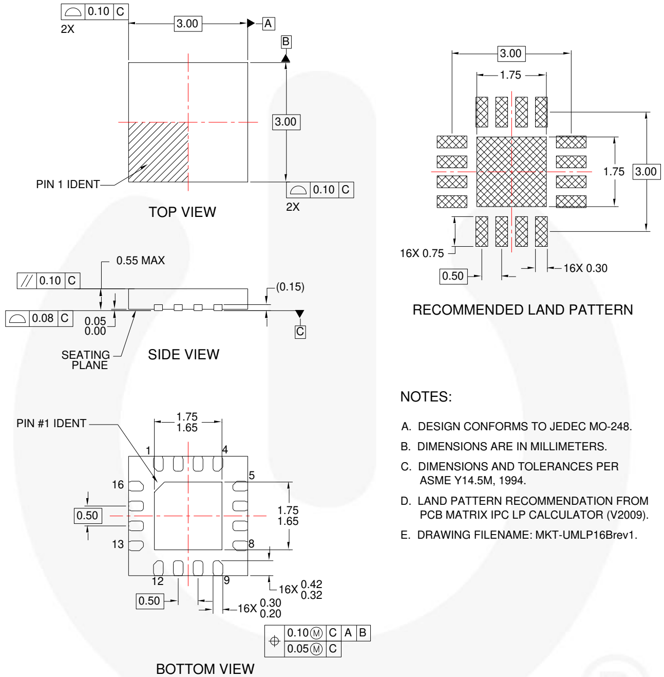
Figure 17. UMLP-16 Dimensions
