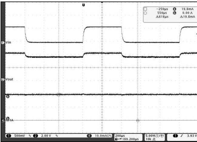
Figure 12. Line Transient Response in 1x Mode, V_{IN}=3.6V - 4.2V , I_{LEDx}=20mA
