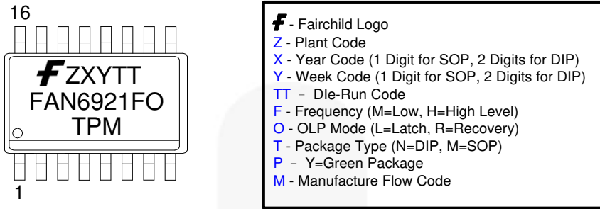
Figure 3. Marking Diagram
