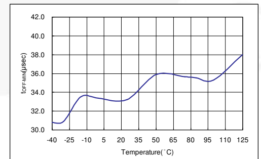
Figure 20. PWM Minimum Off Time for V_{FB} = V_{GN}
