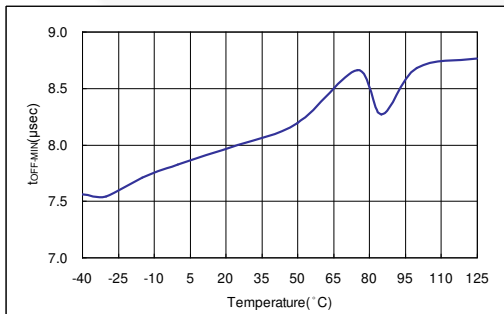
Figure 19. PWM Minimum Off Time for V_{FB} > V_{FN}
