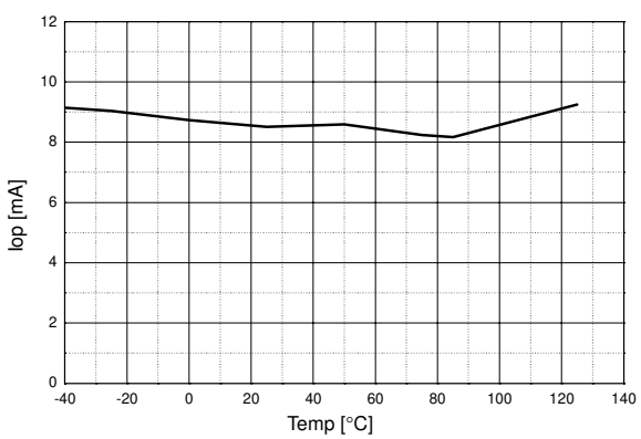
Figure 5. Operating Supply Current
