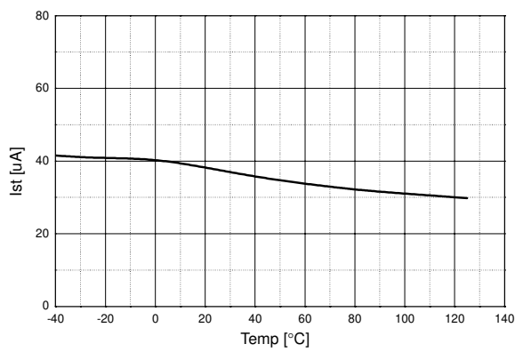
Figure 3. Start up Current
