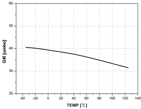
Figure 21. Error Amp. GM vs. Temp.
