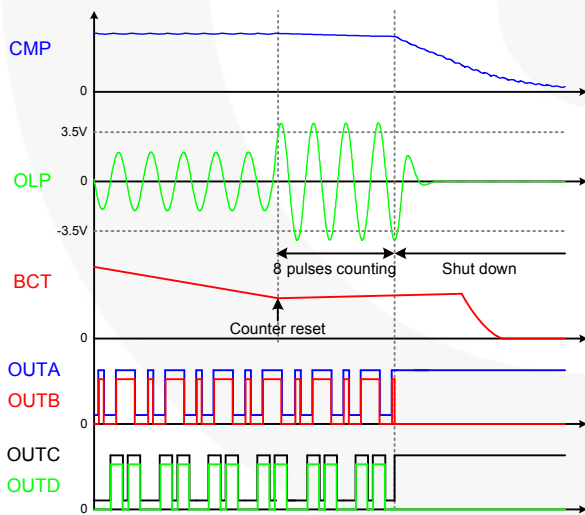
Figure 55. High-FB Protection
