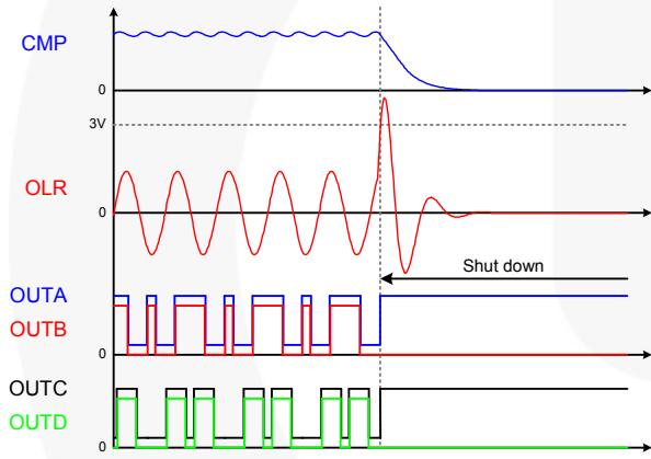
Figure 50. Arc Protection
