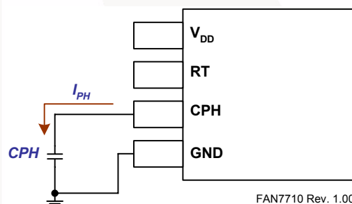
Figure 32. Preheating Timer
