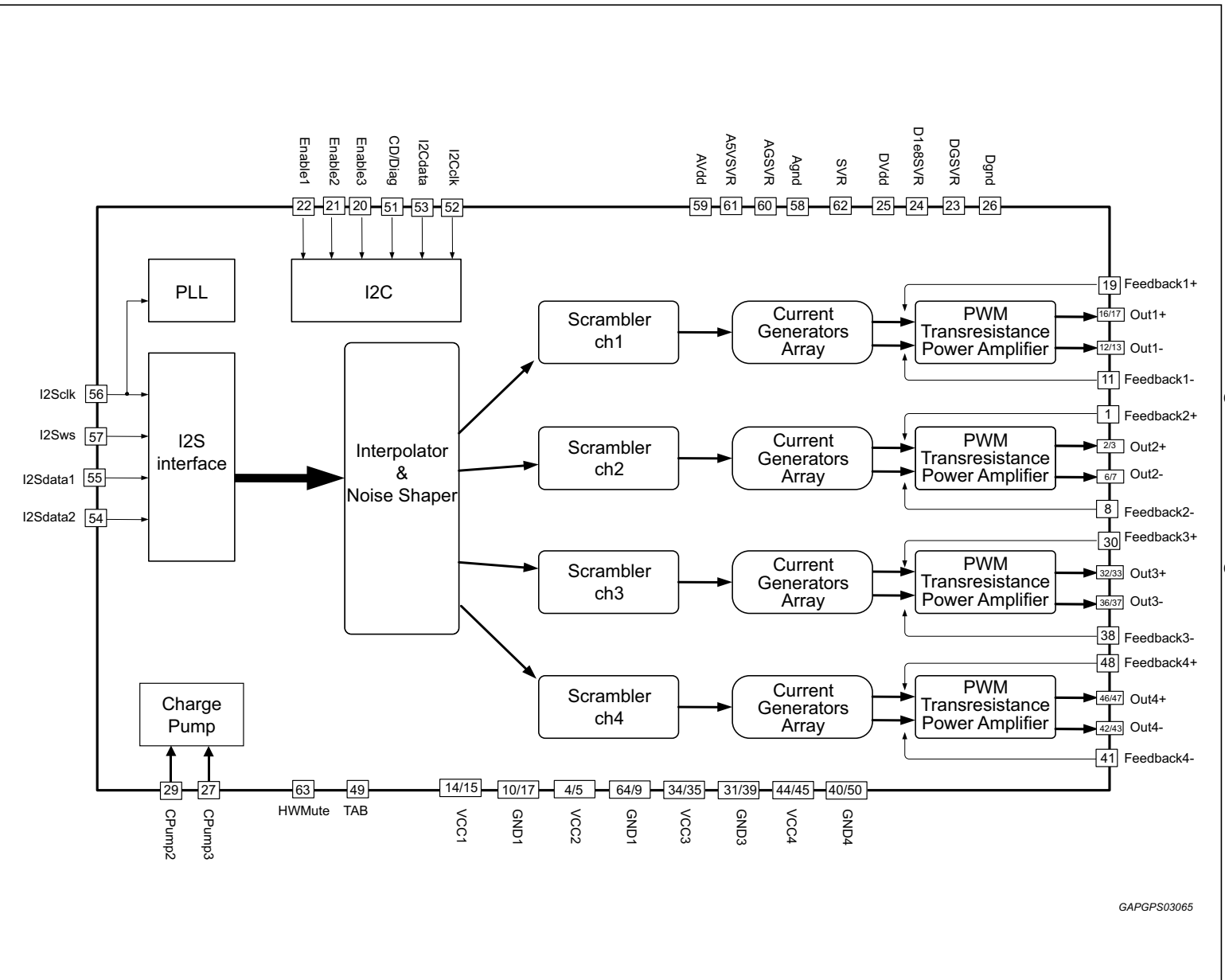
Figure 1. Block diagram
