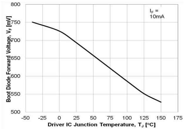
Figure 22. Boot Diode Forward Voltage vs. Temperature
