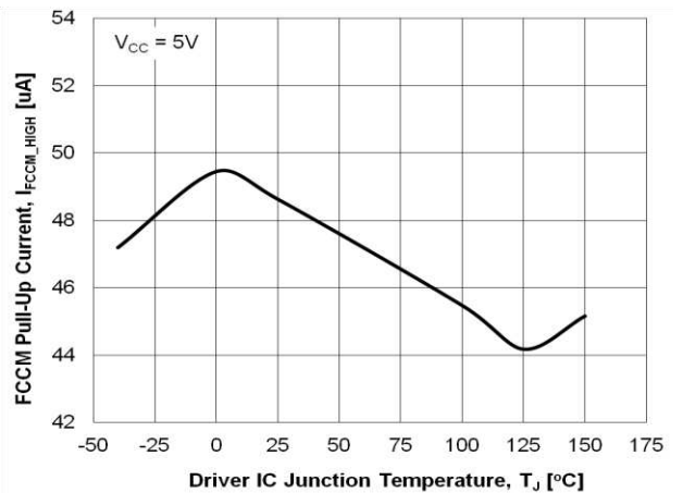
Figure 21. FCCM Pull-Up Current vs. Temperature
