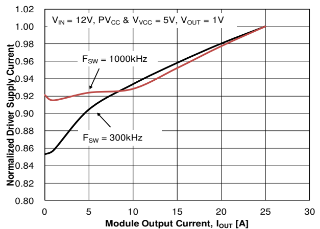
Figure 15. Driver Supply Current vs. Output Current
