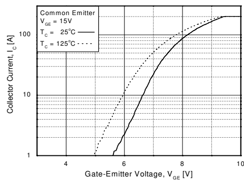
Figure 4. Transfer Characteristics
