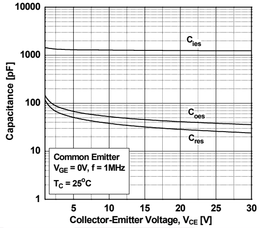
Figure 8. Capacitance Characteristics
