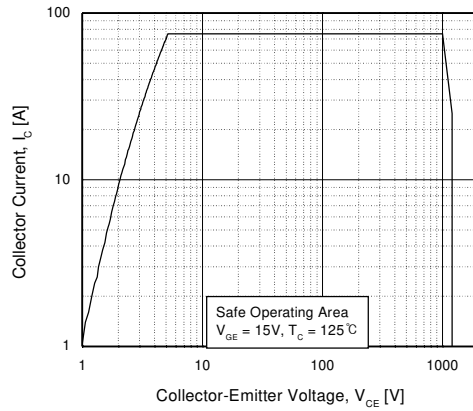
Fig 16. Turn-Off SOA
