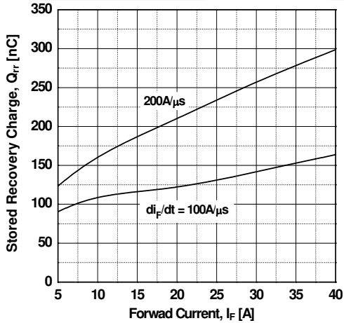
Figure 21. Stored Charge
